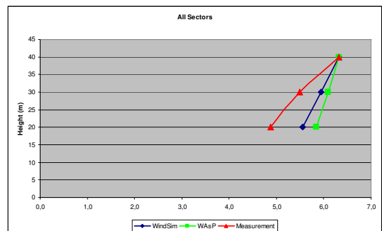
Figure: Vertical profiles k-Parameter CN18
