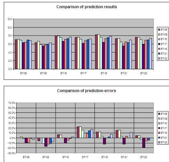
Figures: Computations and computation errors WindSim
